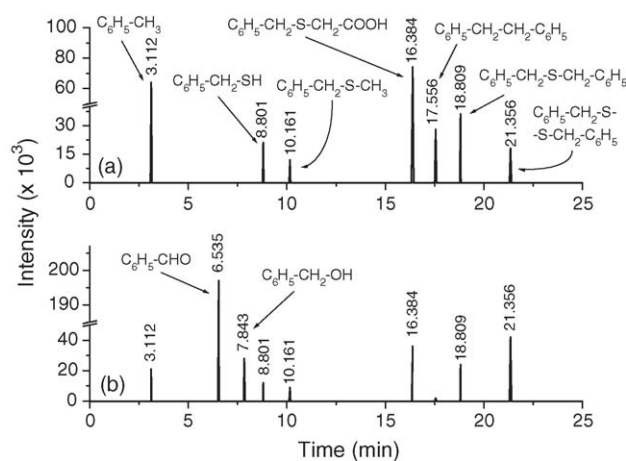
Fig. 3. (a) GC-MS chromatogram recorded after a 75 min irradiation of SBTGA (10 mM) in Ar-saturated acetonitrile. (b) GC-MS chromatogram recorded after an 80 min of irradiation of SBTGA (10 mM) in O 2 -saturated acetonitrile.
