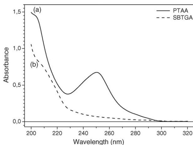
Fig. 1. UV-vis absorption spectra of: (a) 0.1 mM PTAA and (b) 80 \mu M SBTGA in acetonitrile taken in 1 cm UV cell.
